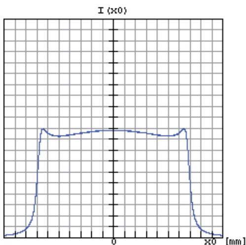
Cylinder lens
