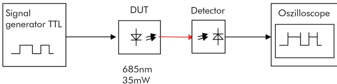
Measuring construction: Peak-value controlled 35 mW laser for operating in a range of CW to 10 MHz.
